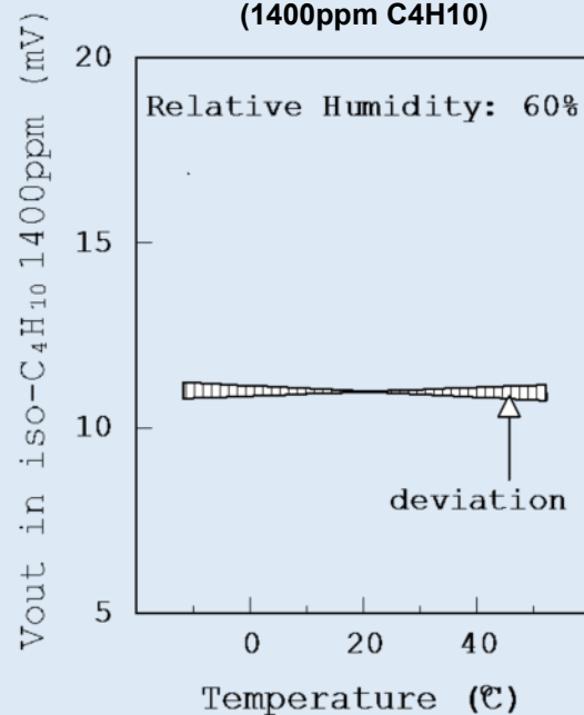
Gas Sensitivity Dependence (1400ppm C 4 H 10 )
